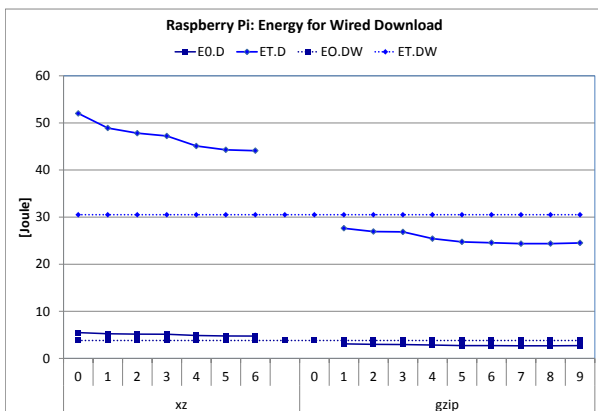
Figure 10. Raspberry Pi: Energy for downloads over Ethernet.
