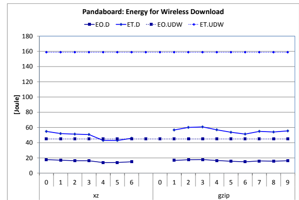
Figure 8. Pandaboard: Energy for download over WLAN.
