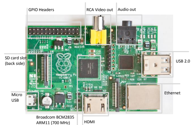
Figure 5. Raspberry Pi.
