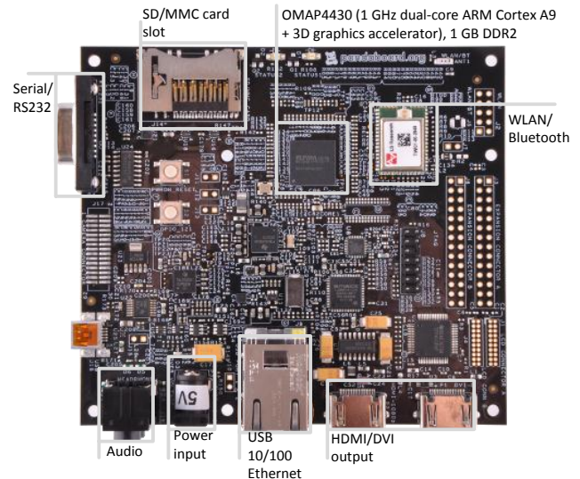
Figure 4. Pandaboard.
