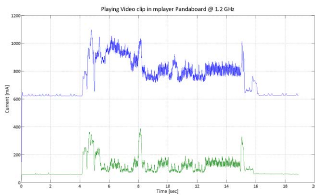
Figure 13. Pandaboard: Current drawn by the platform (blue) and processor core (green) for playing a video clip in mplayer.
