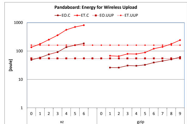
Figure 7. Pandaboard: Energy for upload over WLAN.
