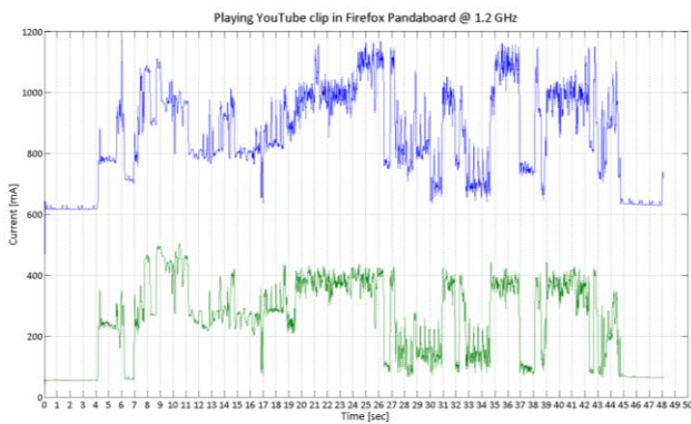
Figure 14. Pandaboard: Current drawn by the platform (blue) and processor core (green) for playing a Youtube video clip in Firefox.
