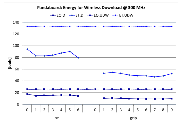
Figure 12. Pandaboard: Energy for downloads over WLAN @300 MHz processor clock.
