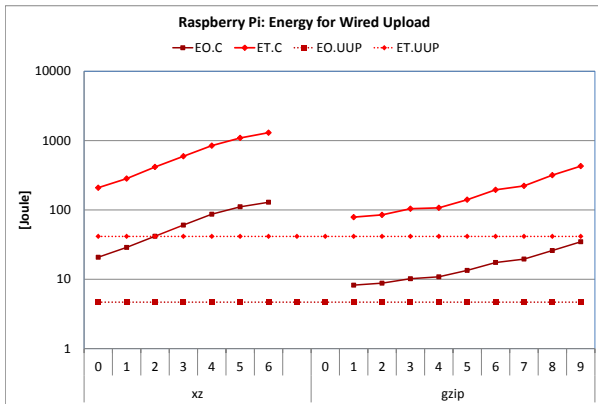
Figure 9. Raspberry Pi: Energy for uploads over Ethernet.
