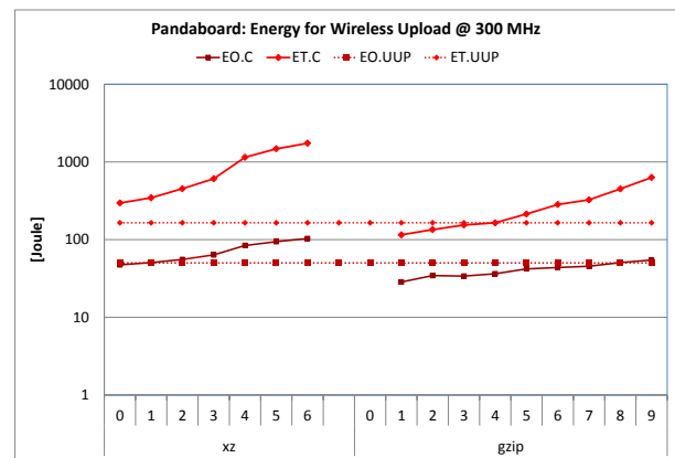
Figure 11. Pandaboard: Energy for uploads over WLAN at 300 MHz processor clock.
