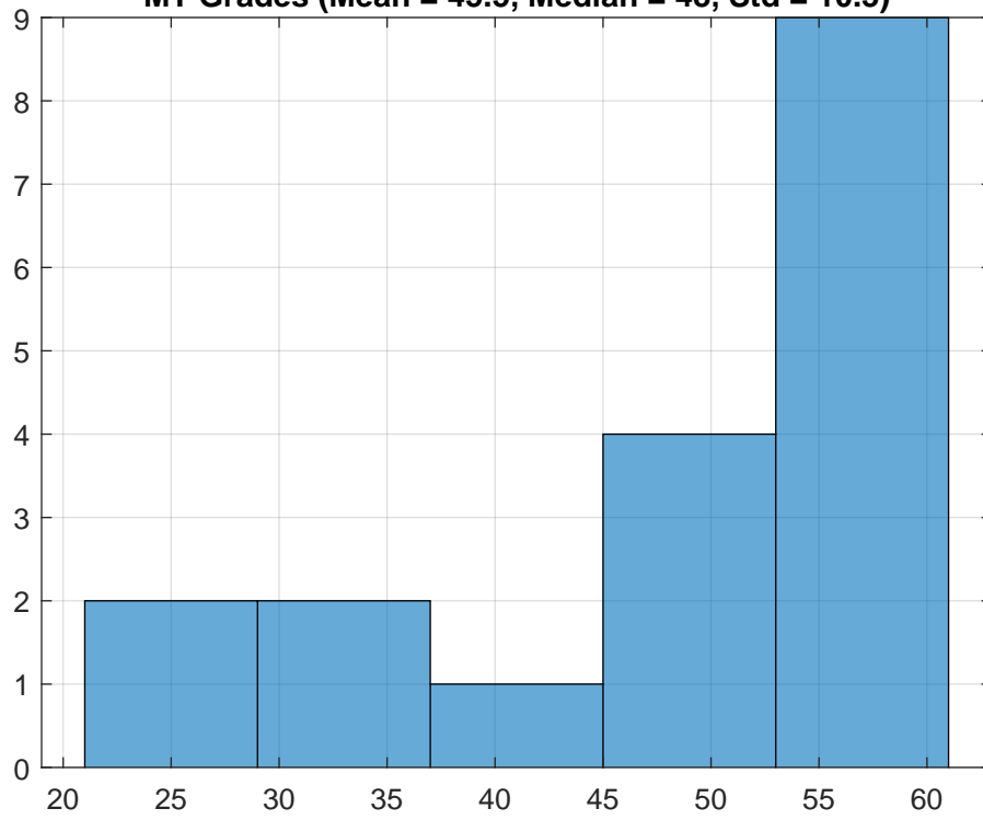
MT Grades (Mean = 45.5, Median = 48, Std = 10.3)
