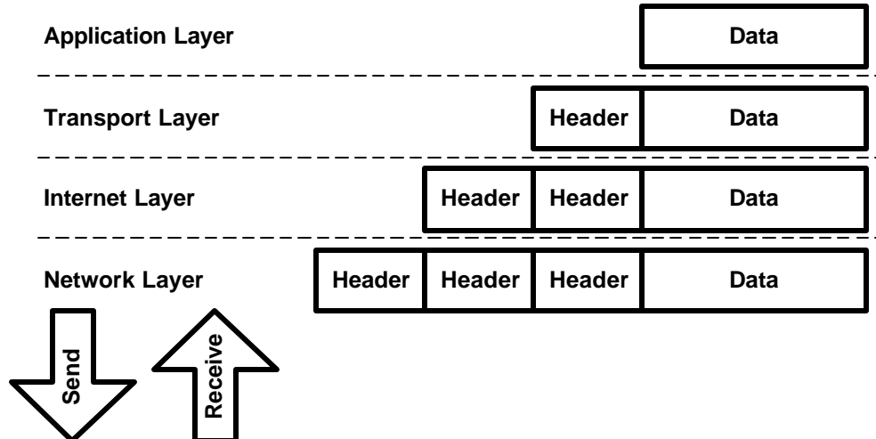
Figure 2. Data Encapsulation
