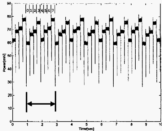
Fig. 7. Power traces the CntToLedsAndRfm application under TinyOS running on a Telos A platform.
