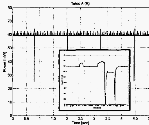
Fig. 10. Power traces for the Testera TinyOS application running on Telos A measured by the shunt resistor.
