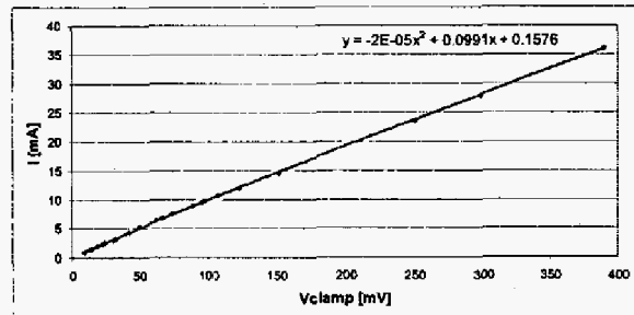
Fig. 4. Current probe calibration.
