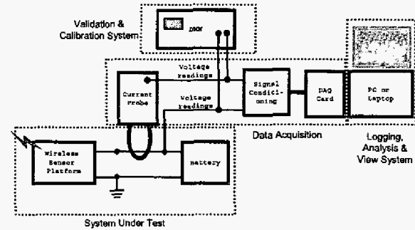
Fig. 2 Block diagram of the environment for run-time power monitoring for wireless sensor platforms. Description: DMM – Digital Multimeter, DAQ – Data Acquisition Card.
