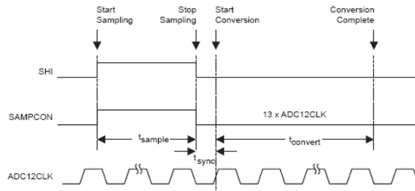
Figure 17-3. Extended Sample Mode
