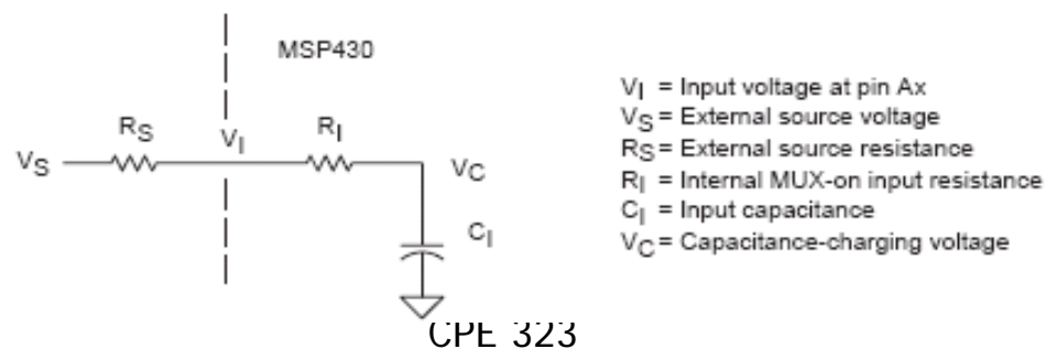
Figure 17-5. Analog Input Equivalent Circuit
