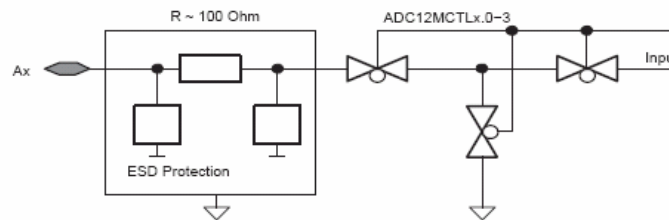
Figure 17-2. Analog Multiplexer
