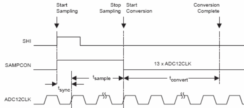
Figure 17-4. Pulse Sample Mode
